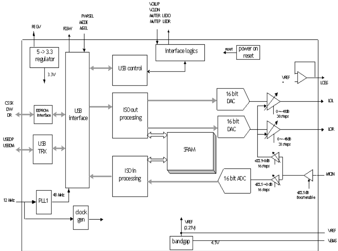
Block Diagram Of HS-100
